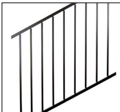
Top / bottom rail measure 1-1/4" x 1-1/4" 5/8" Square Infill Adjustable from 30° - 40°
