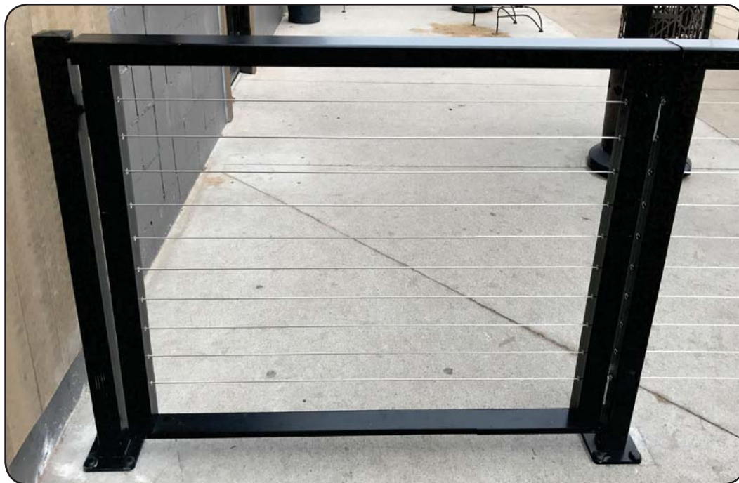
Completed Gate Assembly (Latch & Hinge on Opposite Side)
